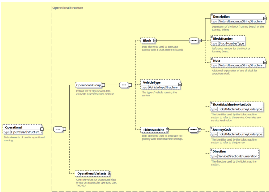
Figure 32 - The OperationalStructure supporting real time elements
