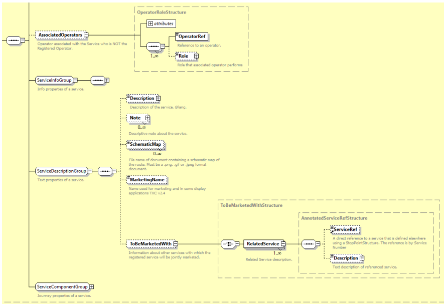
Figure 11 - Excerpt from Service element showing association elements
