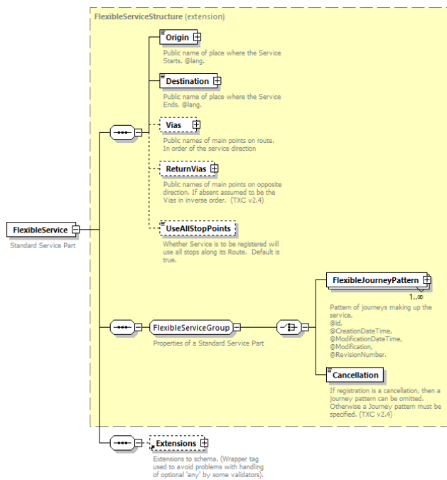
Figure 34 - The FlexibleService element
