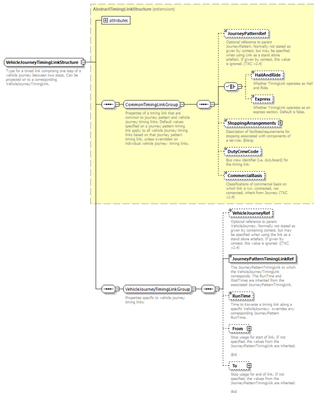
Figure 30 - The VehicleJourneyTimingLink structure
