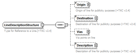
Figure 15 - The line description structure
