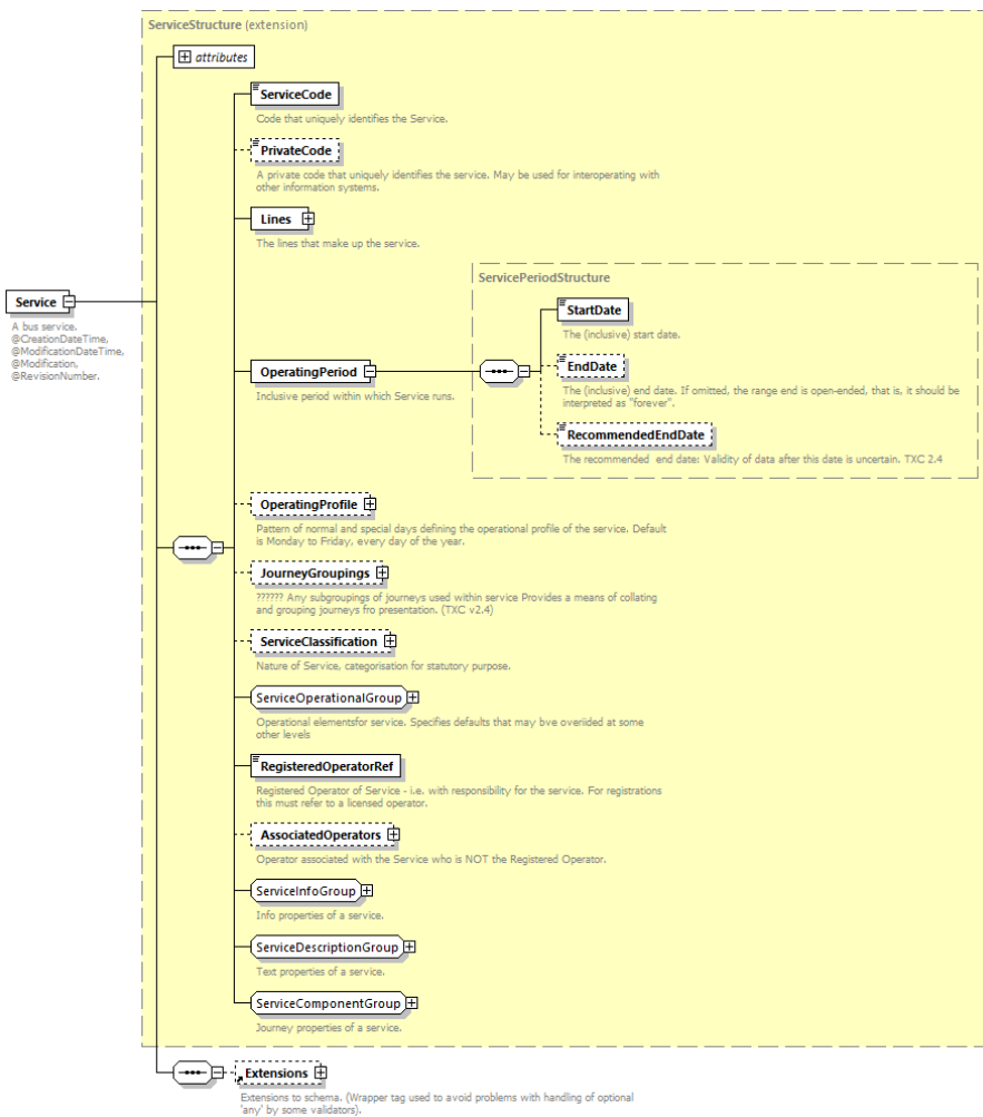
Figure 10 - The Service element
