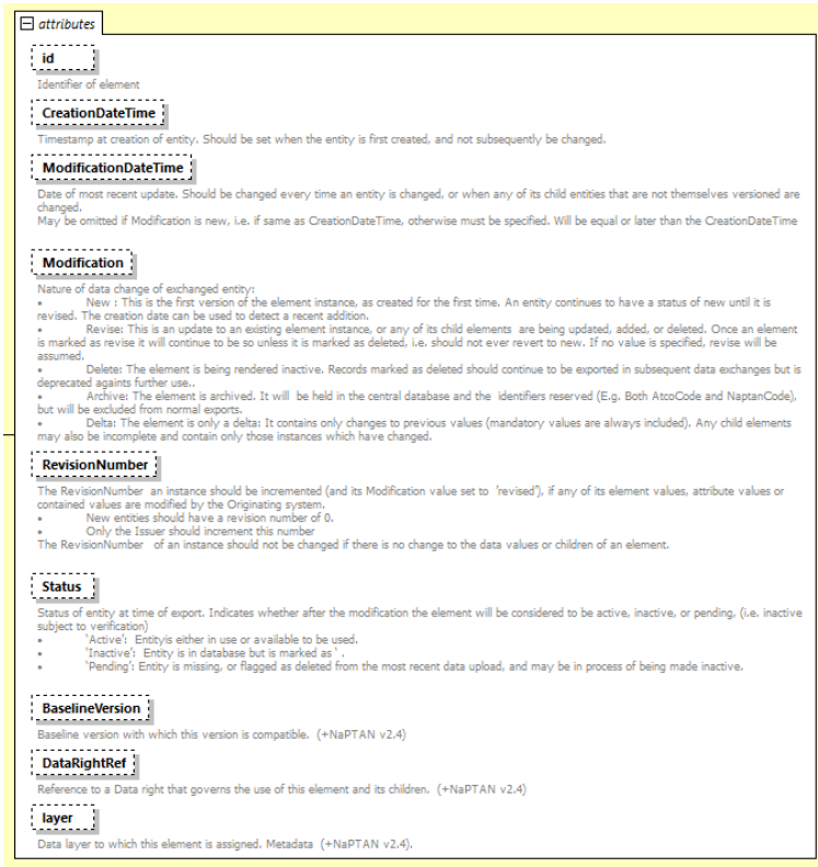
Figure 1 - An indicative set of element attributes
