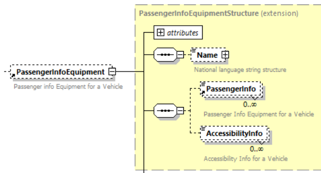
Figure 3 - The PassengerInfoEquipment element
