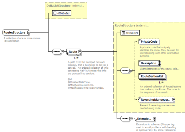
Figure 19 - The Routes structure
