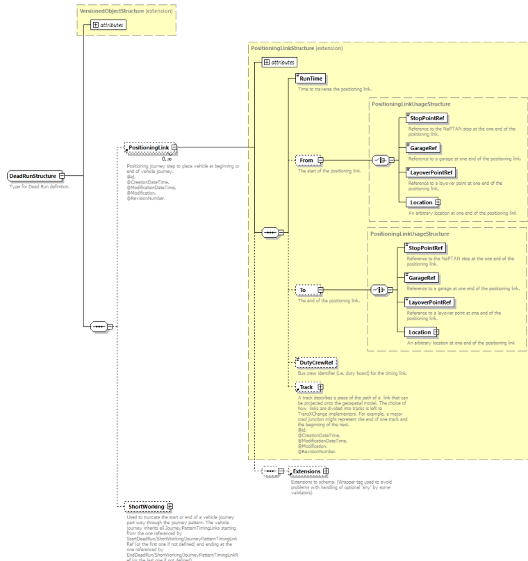
Figure 33 - The DeadRun structure
