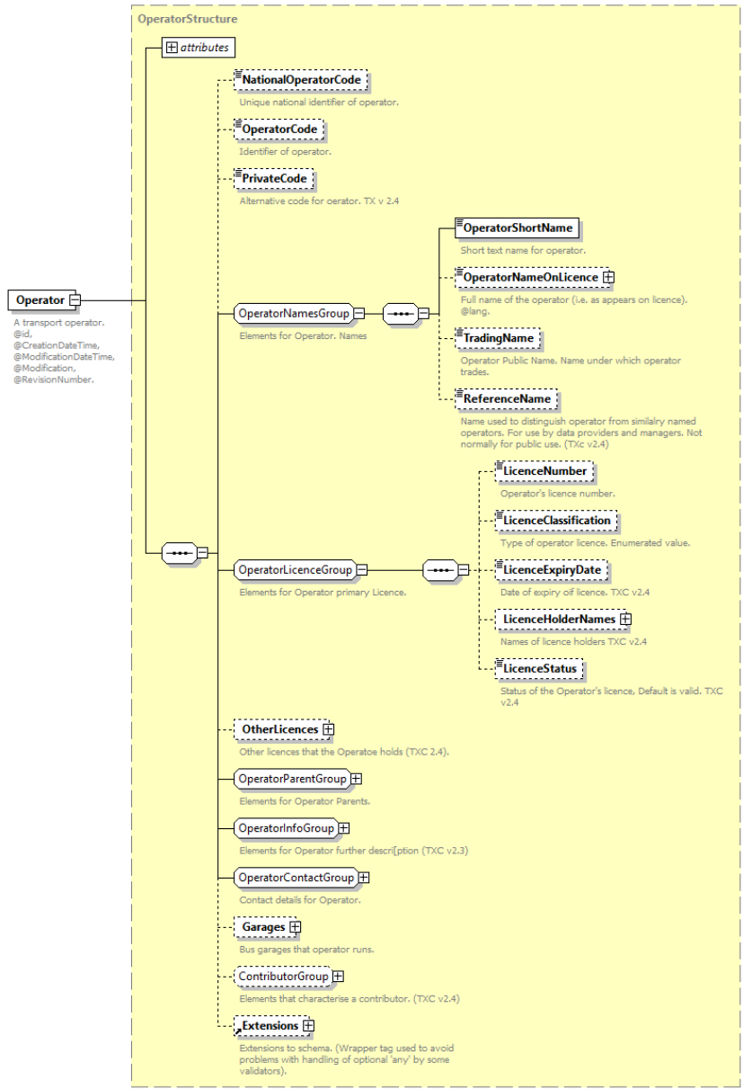
Figure 9 - The Operator element
