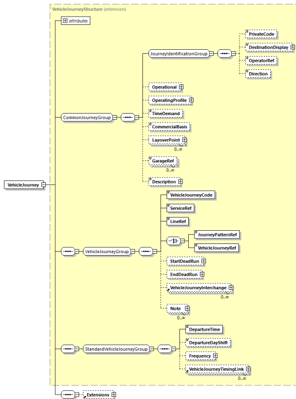
Figure 25 - Basic structure of a VehicleJourney
