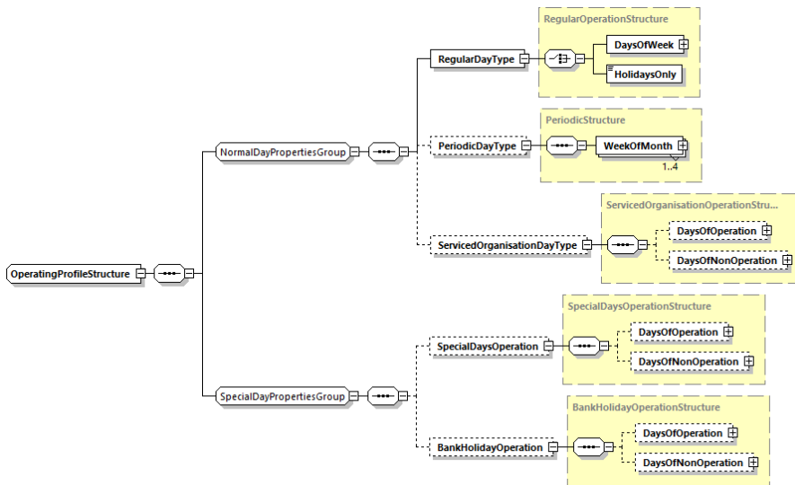
Figure 26 - Basic structure of an OperatingProfile
