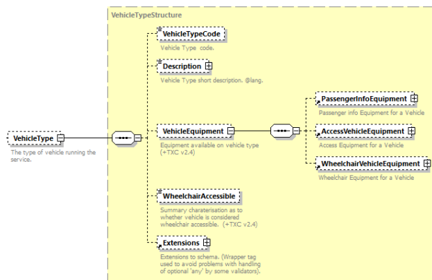
Figure 2 - The VehicleType structure
