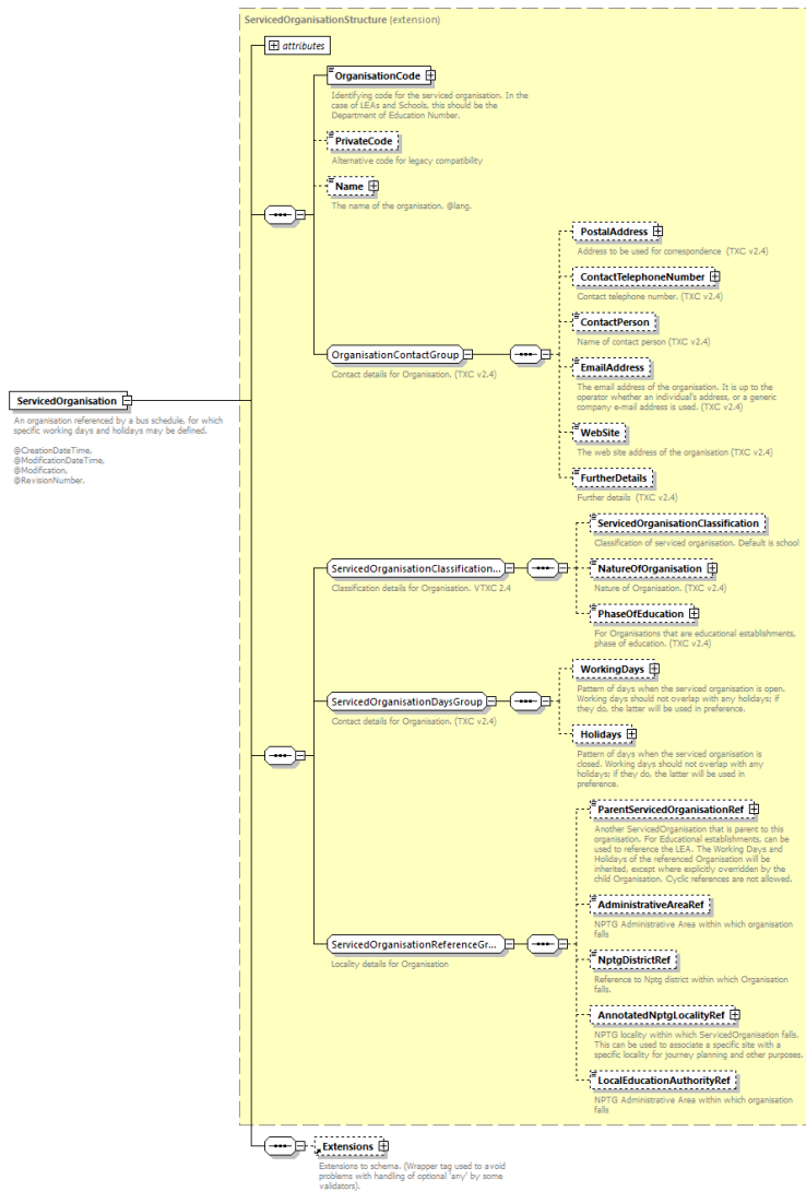
Figure 7 - The ServicedOrganisation element
