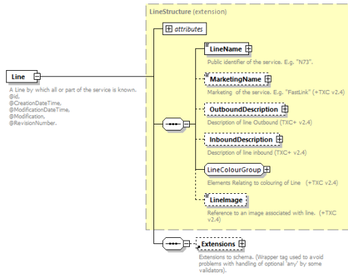
Figure 14 - The Line element
