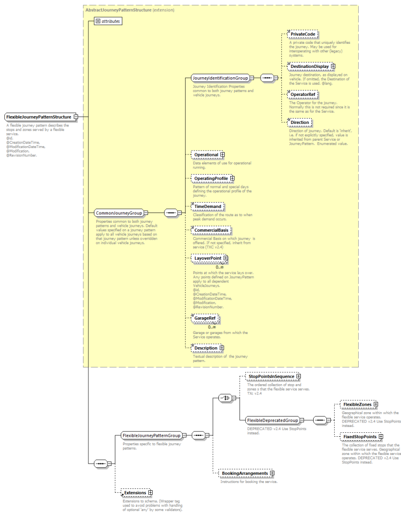
Figure 35 - The flexible journey pattern structure
