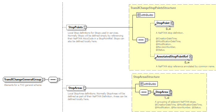
Figure 16 - StopPoints and StopAreas in a TxC document
