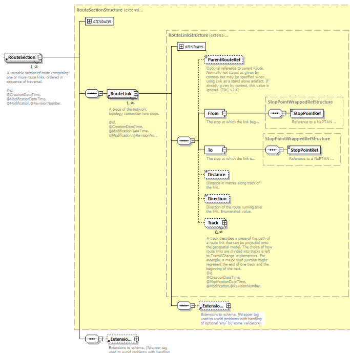
Figure 20 - RouteSection and RouteLink structure
