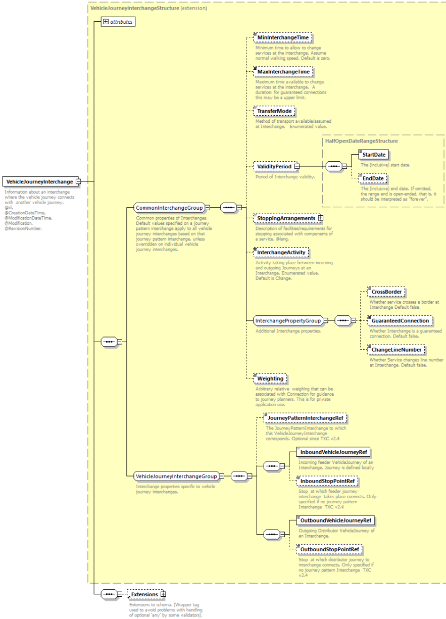
Figure 31 - The VehicleJourneyInterchange element
