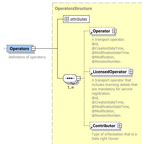
Figure 8 - The Operators structure
