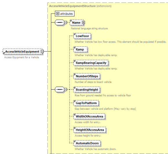
Figure 4 - The AccessVehicleEquipment element
