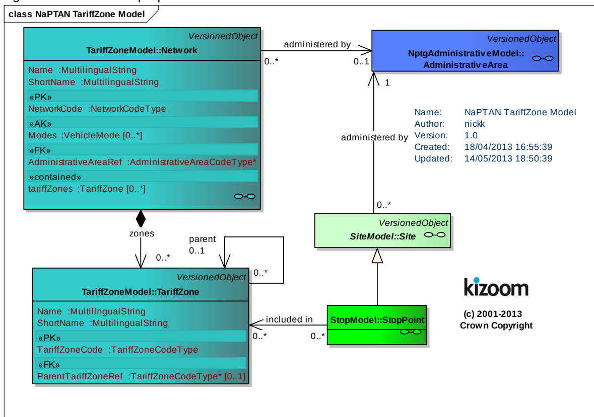
Figure 3-22 – UML Diagram of NaPTAN TariffZones – Details
