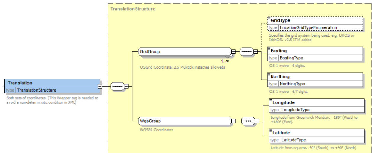
Figure 8-2 – Translation Element
