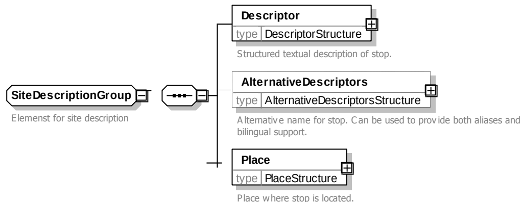
Figure 6-5 – SiteDescriptionGroup Group
