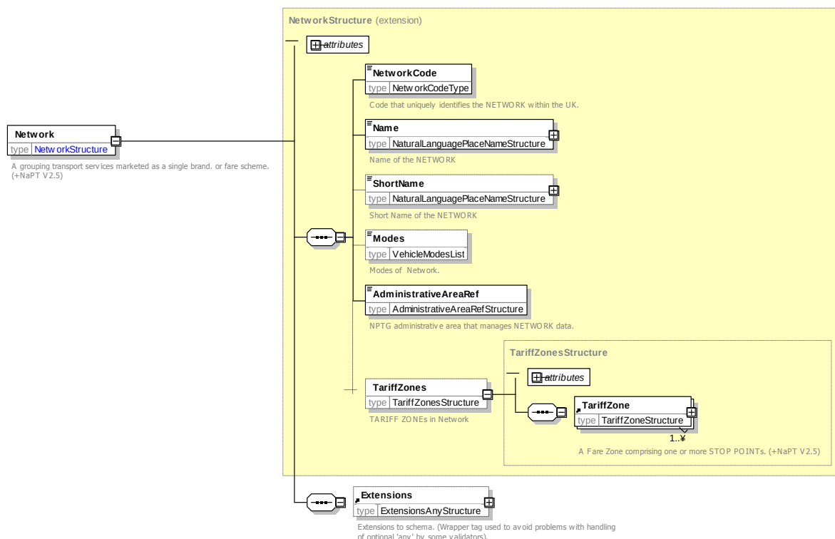
Figure 6-32 – Network Element
