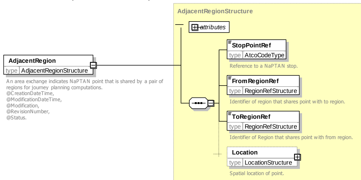
Figure 7-6 – AdjacentRegionPoint Element
