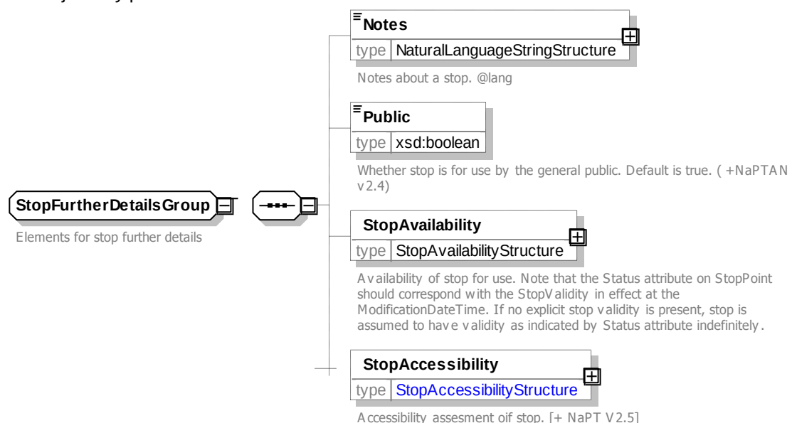
Figure 6-9 – StopFurtherDetailsGroup Group
