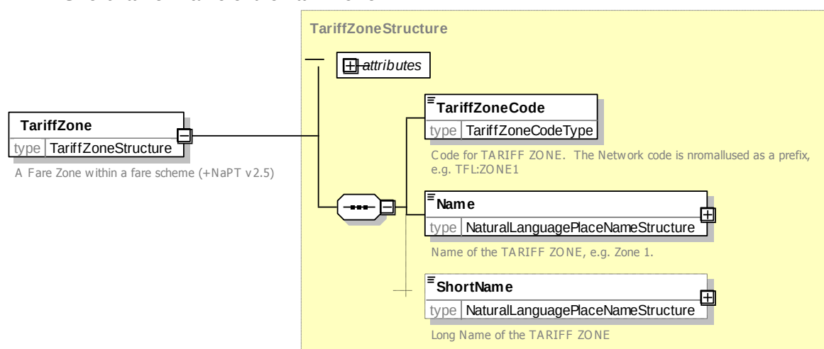
Figure 6-33 – TariffZone Element
