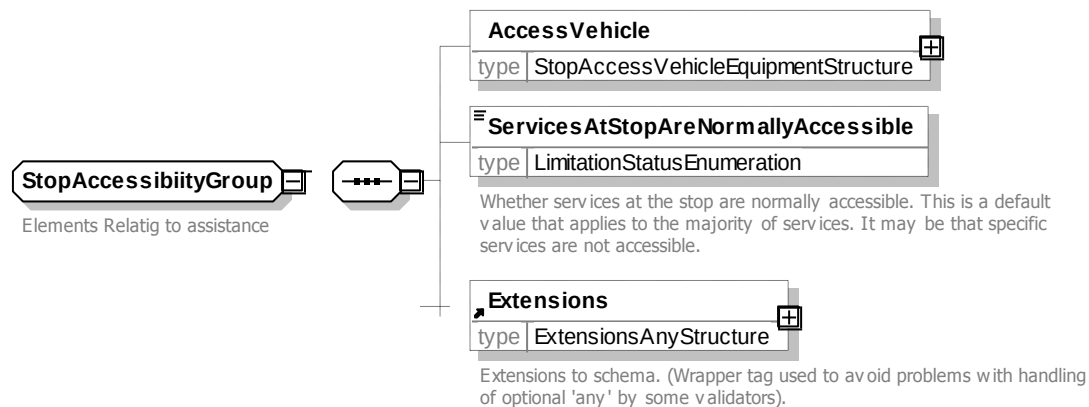
Figure 6-27 – StopAccessibilityGroup Group
