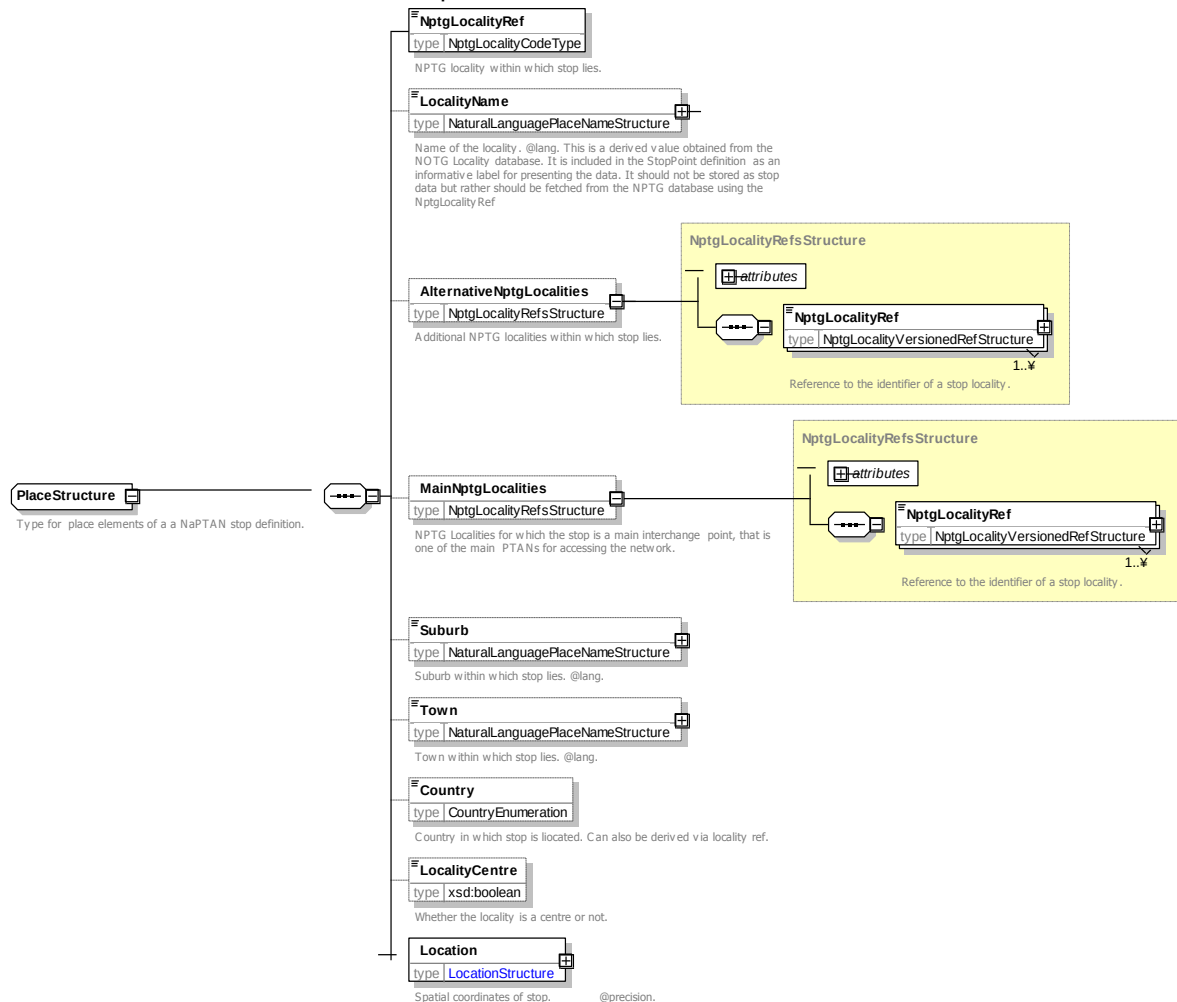
Figure 6-7 – Place Element
