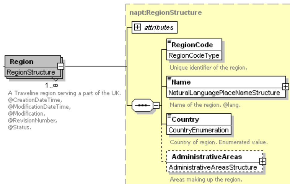
Figure 5-3 – Region Element
