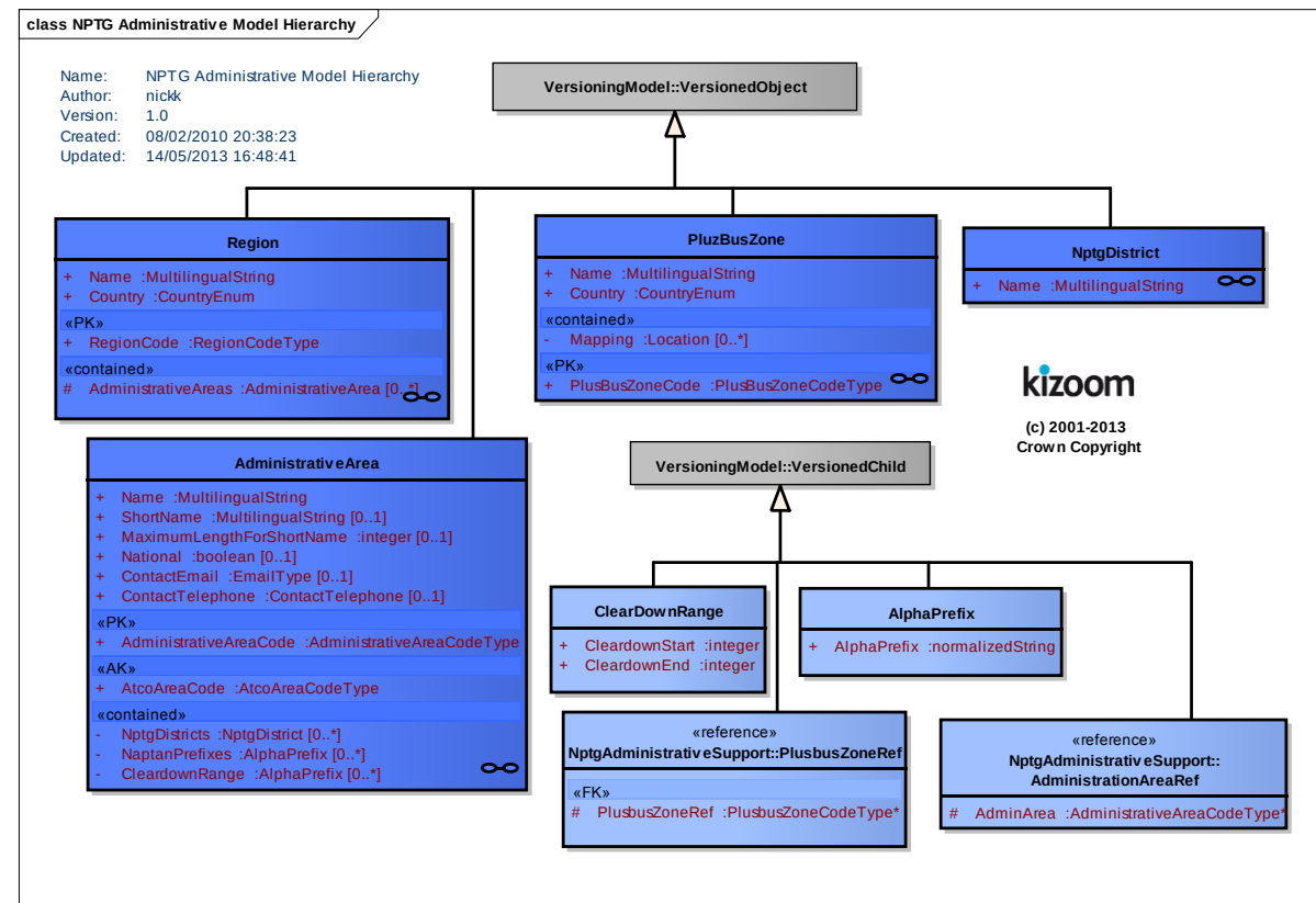
Figure 3-7 – UML Diagram of Administrative Element Hierarchy
