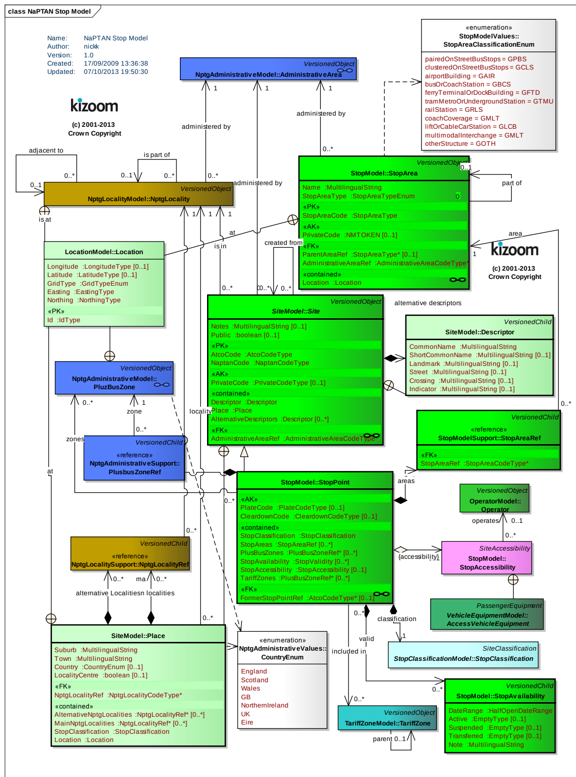
Figure 3-16 – UML Diagram of NaPTAN Model: Detail
