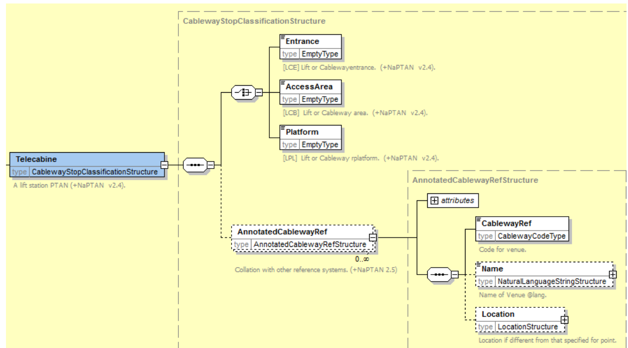
Figure 6-23 – OffStreet / Telecabine Element
