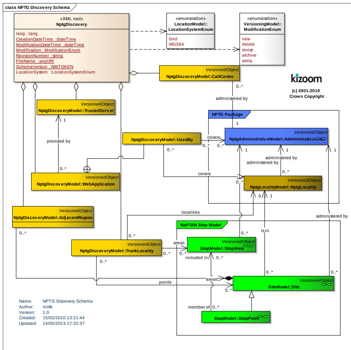
Figure 7-1 – UML Diagram of the NPTG Discovery Schema
