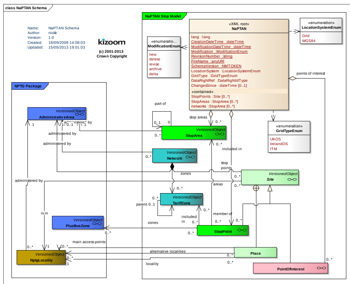
Figure 6-1 – UML Diagram of NaPTAN Schema
