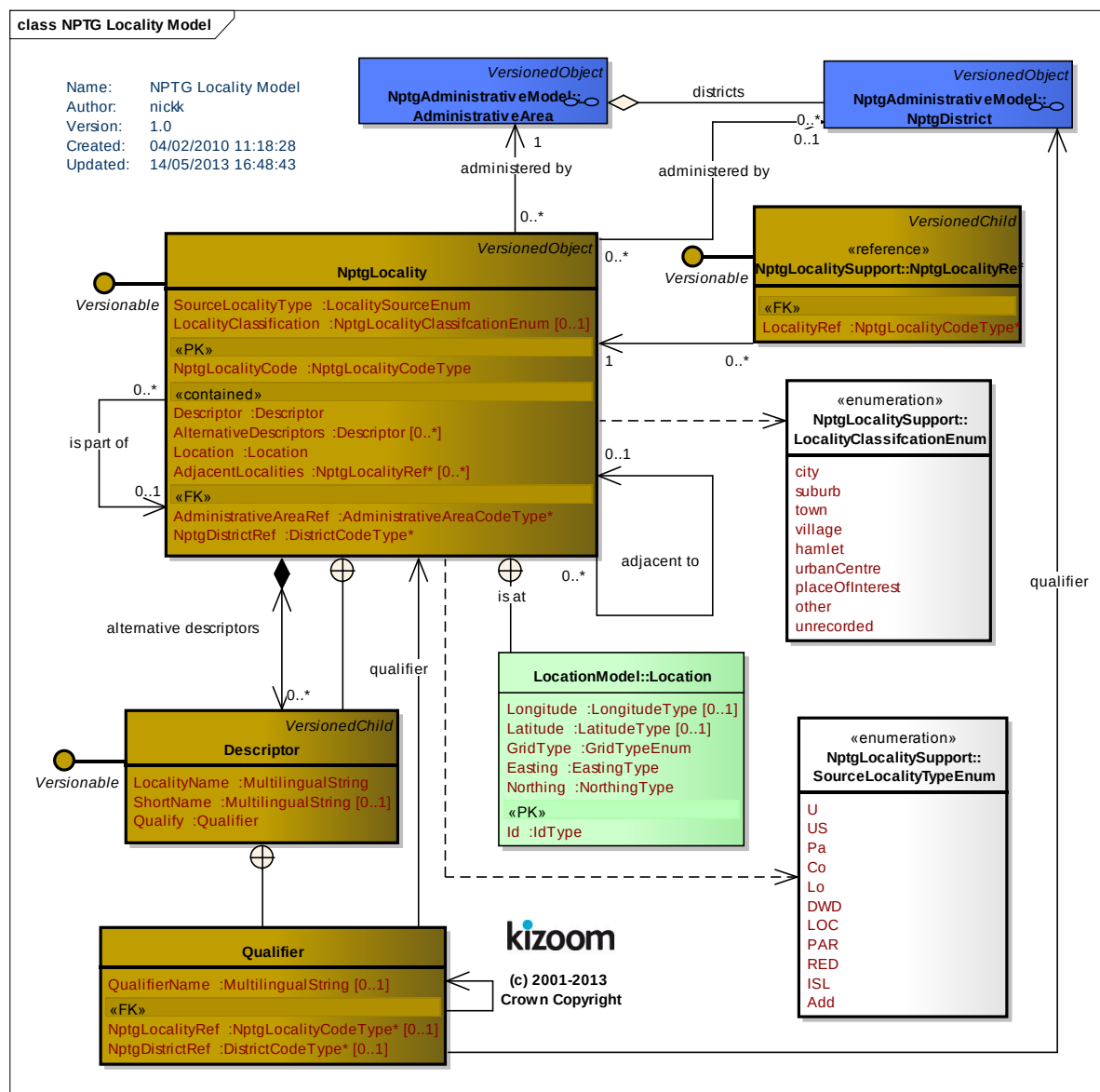
Figure 3-2 – UML Diagram of NPTG Locality Model
