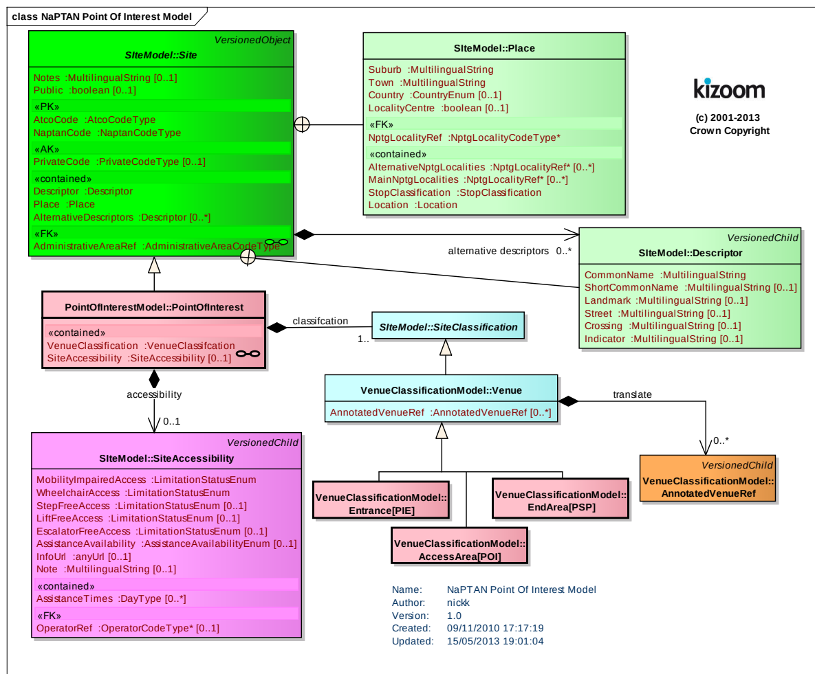
Figure 3-24 – UML Diagram of NaPTAN PointOfInterest - Details
