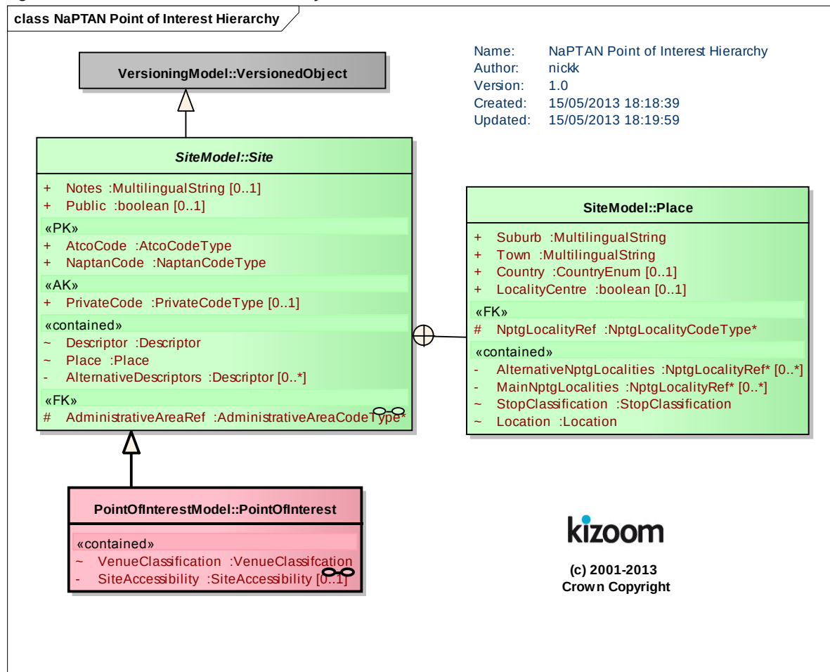
Figure 3-27 – UML Diagram of NaPTAN PointOfInterest Hierarchy
