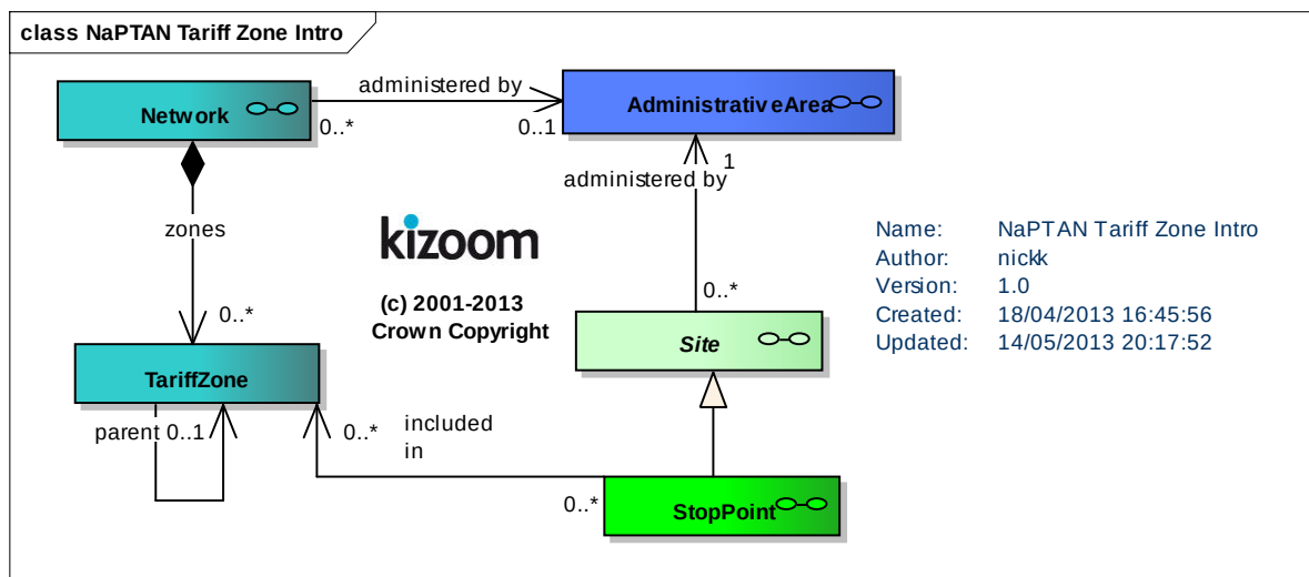
Figure 3-21 – UML Diagram of NaPTAN TariffZones - Overview
