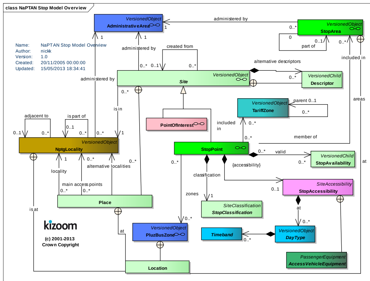
Figure 3-15 – UML Diagram of NaPTAN Model: Overview
