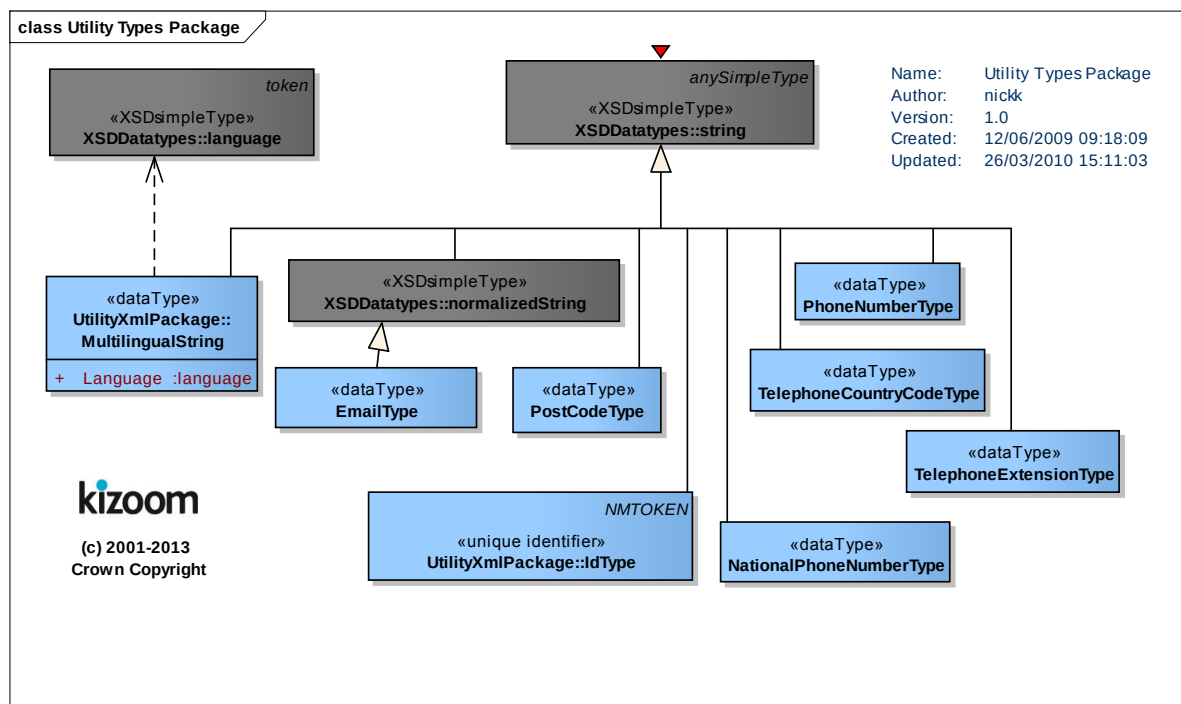
Figure 3-11 – UML Diagram of NaPT Utility Data Types
