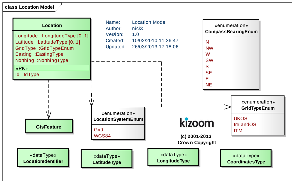
Figure 3-10 – UML Diagram of Location Data Types
