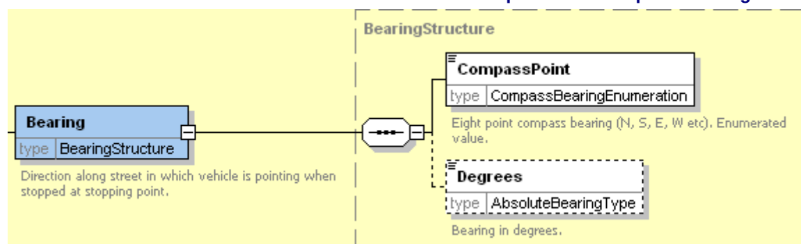
Figure 8-3 – Bearing Element
