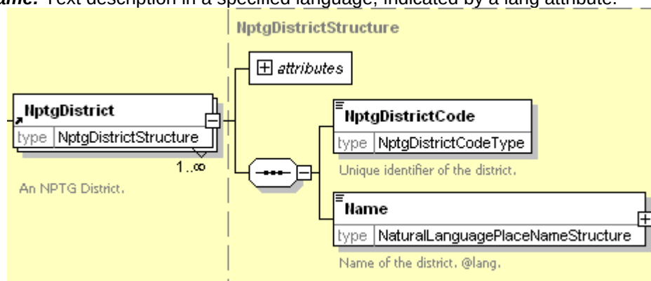
Figure 5-7 – NptgDistrict Element
