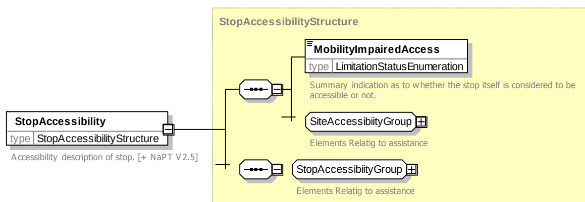
Figure 6-25 – StopAccessibility Element
