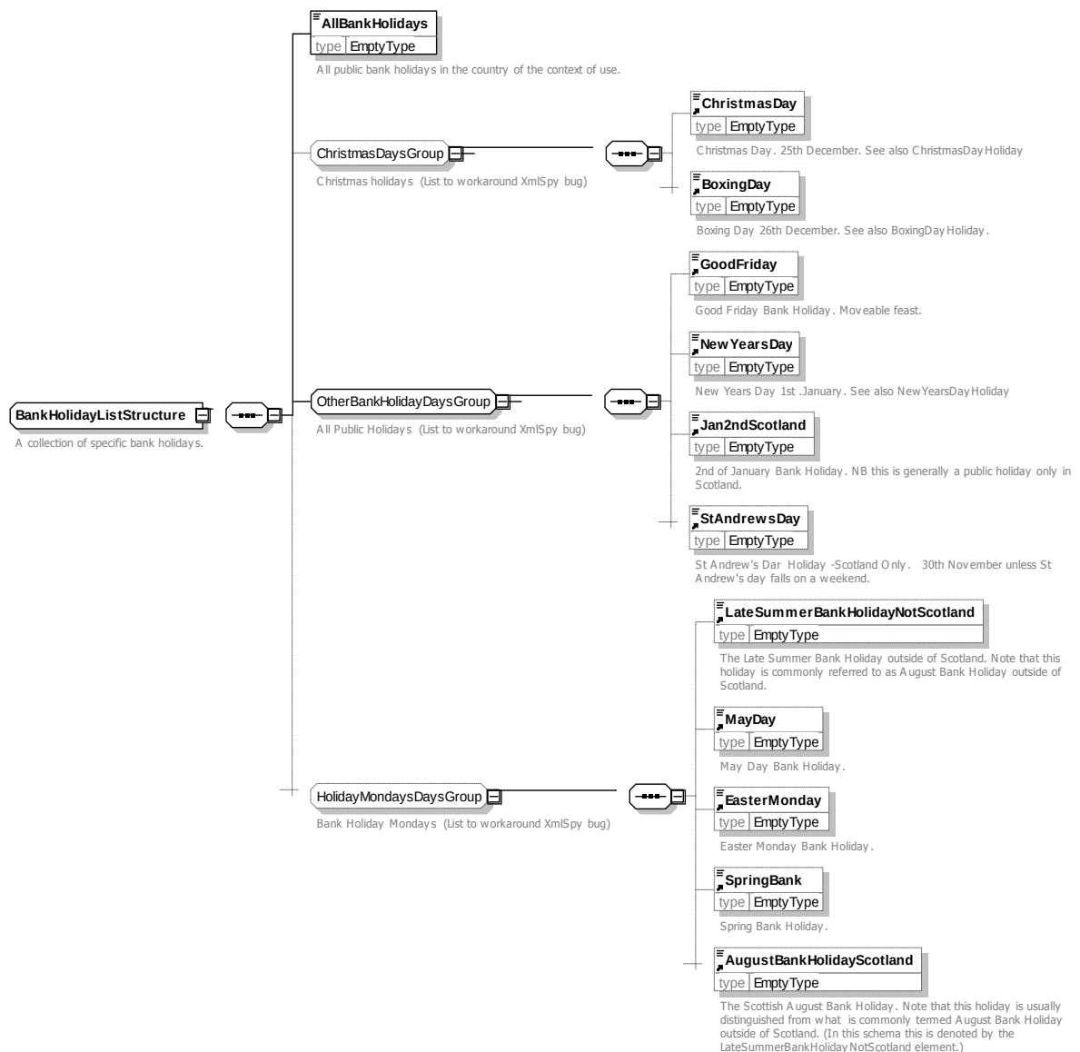
Figure 6-30 – BankHolidays Element
