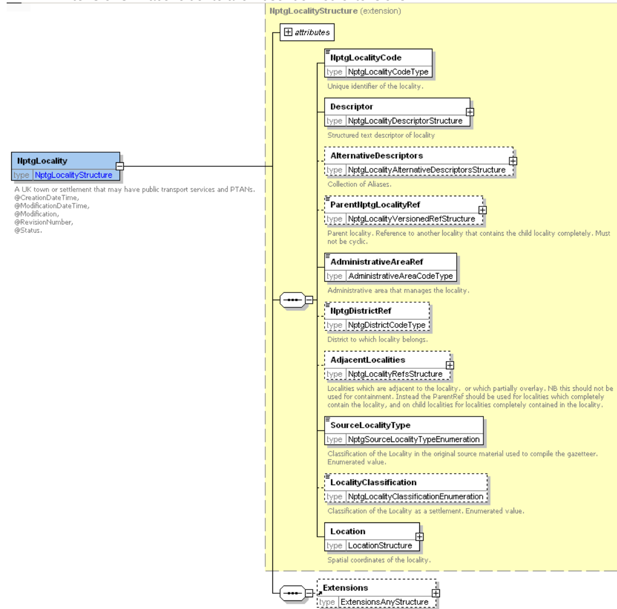
Figure 5-5 – NptgLocality Element
