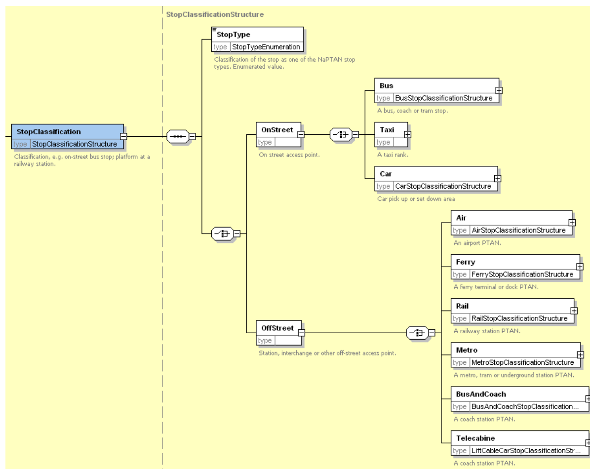
Figure 6-10 – StopClassification Element
