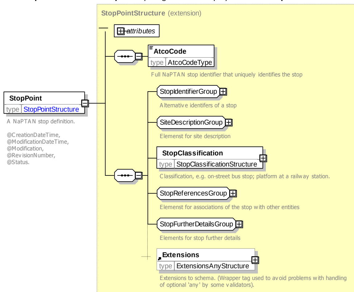
Figure 6-3 – StopPoint Element
