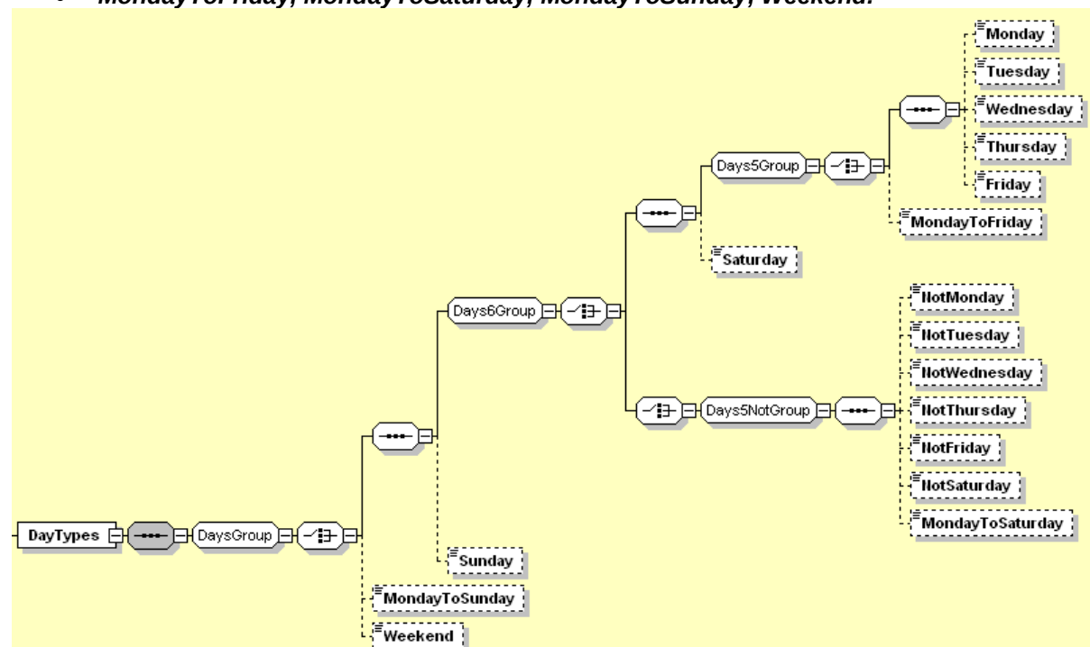
Figure 7-9 – DayTypes Element
