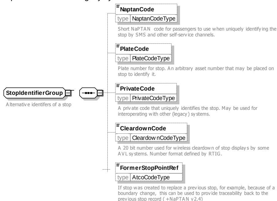
Figure 6-4 – StopIdentifierGroup Group
