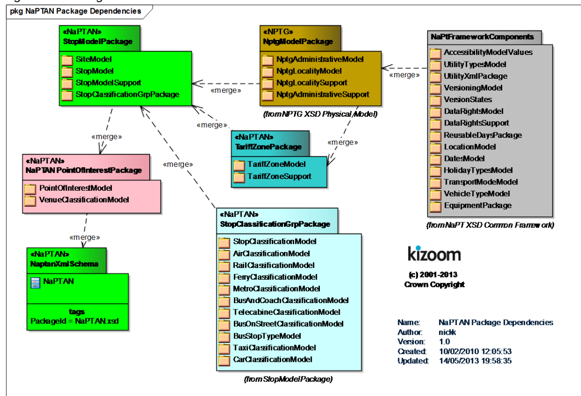
Figure 11-9 – NaPTAN Packages
