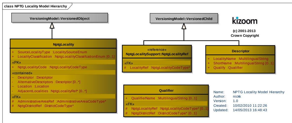
Figure 3-6 – UML Diagram of NPTG Locality Element Hierarchy
