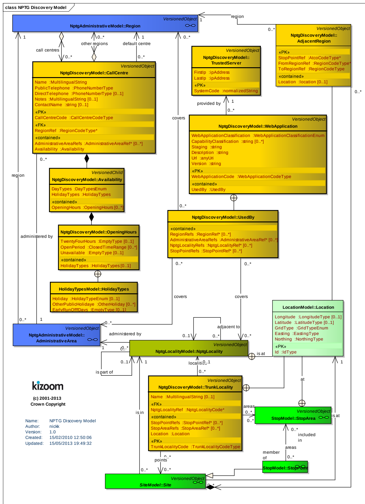
Figure 3-32 – UML Diagram of Discovery Model: Detail
