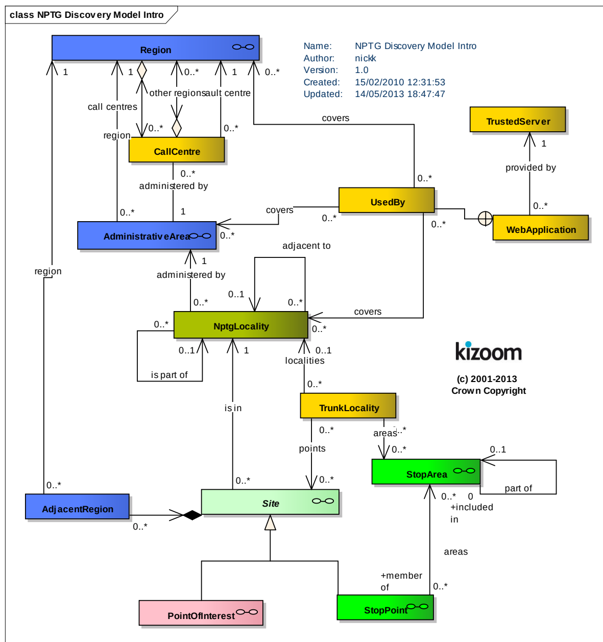
Figure 3-31 – UML Diagram of Discovery Model: Overview
