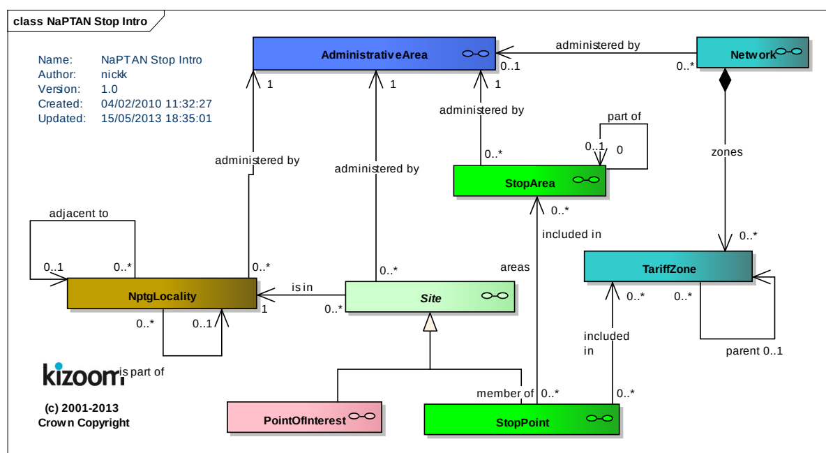
Figure 3-14 – UML Diagram of primary NaPTAN elements
