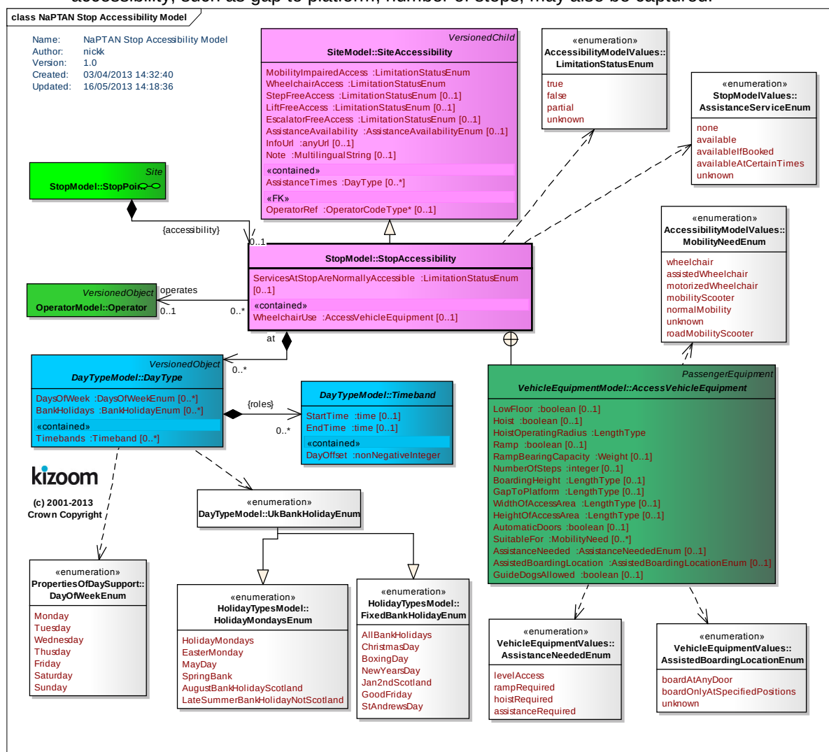
Figure 3-20 – UML Diagram of NaPTAN StopAccessibility
