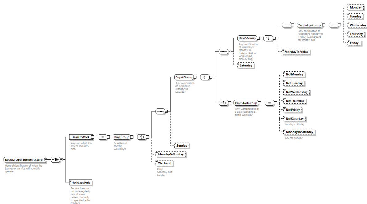
Figure 27 - The RegularOperationStructure
