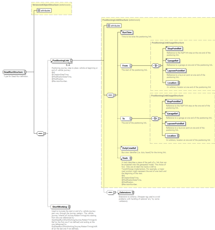
Figure 33 - The DeadRun structure
