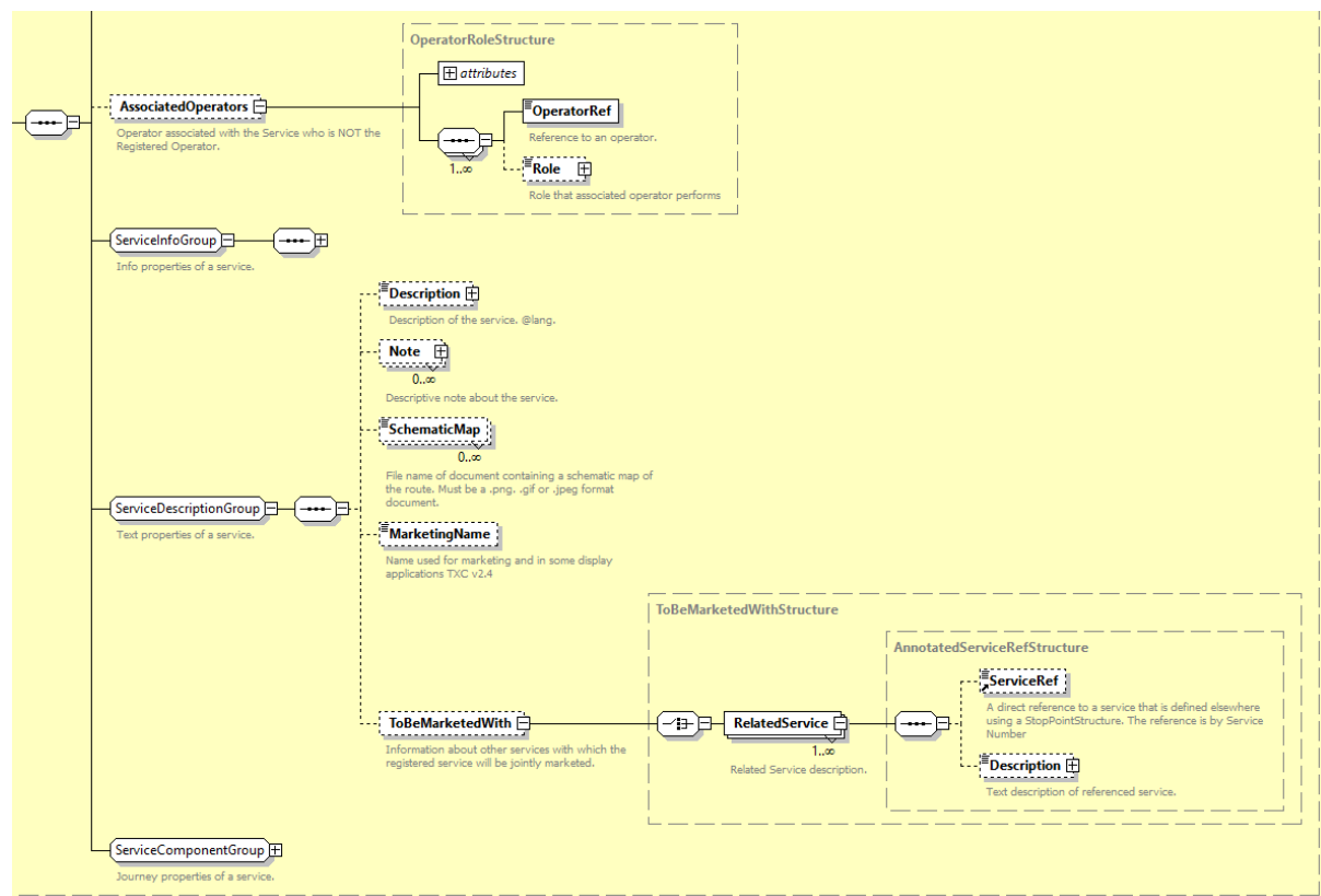
Figure 11 - Excerpt from Service element showing association elements
