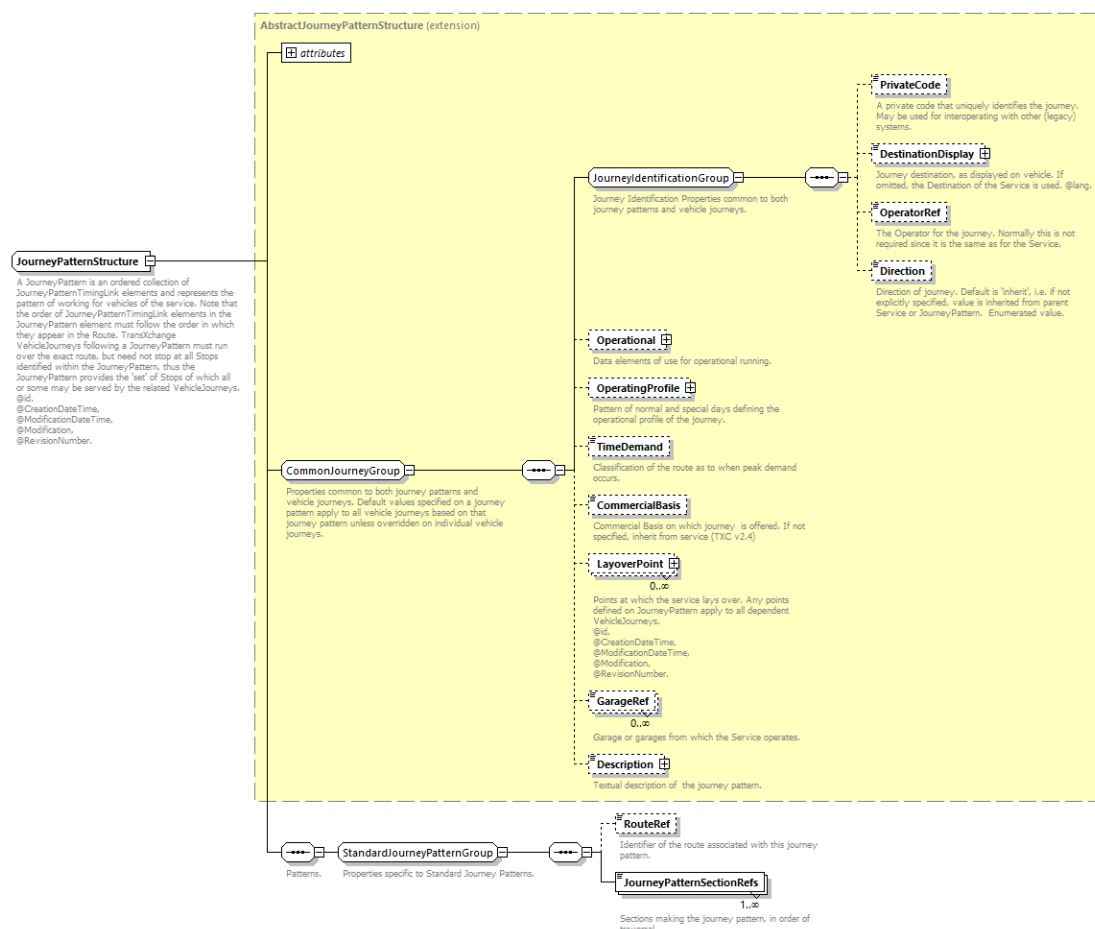
Figure 22 - The JourneyPattern structure
