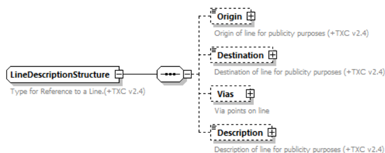
Figure 15 - The line description structure
